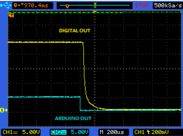
PWM Waveform:
